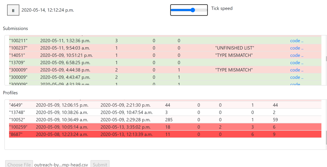
Figure 4: Screenshot of a prototype dashboard that mentors could use to gain real-time insights about students. The "Submission" section presents real-time compiles, code insights, and the compilation status. The "Profile" section uses aggregate statistics to inform the mentors of a student's compilation history; the more red a student's profile is, the more unsuccessful compiles they've had. The "Tick Speed" and pause controls are used to control playback of the historical data on compile errors, and would not be part of the real dashboard.
